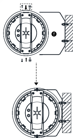
Surface / Ceiling Mounting
